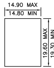
Single Panel-Latch Clearance Panel Thickness 1.60mm
